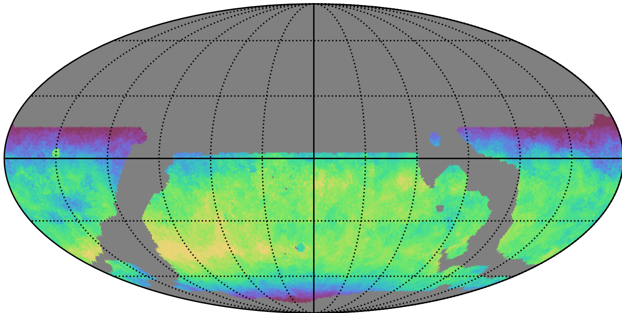
weather_cloudso12v3.4_10yrs WFD y band: Median skyBrightness
