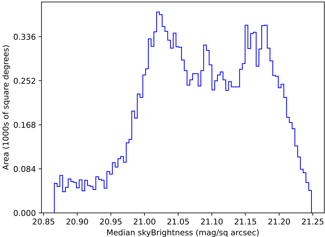
weather_cloudso12v3.4_10yrs WFD r band: Median skyBrightness
