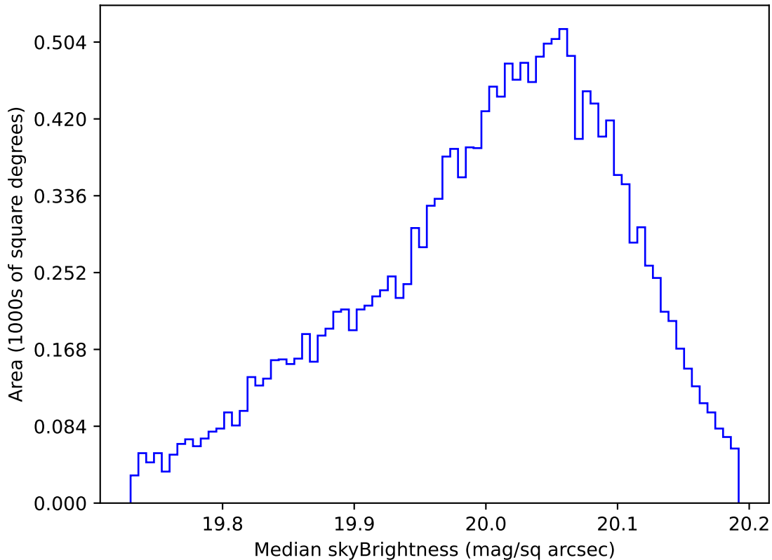
weather_cloudso12v3.4_10yrs WFD i band: Median skyBrightness
