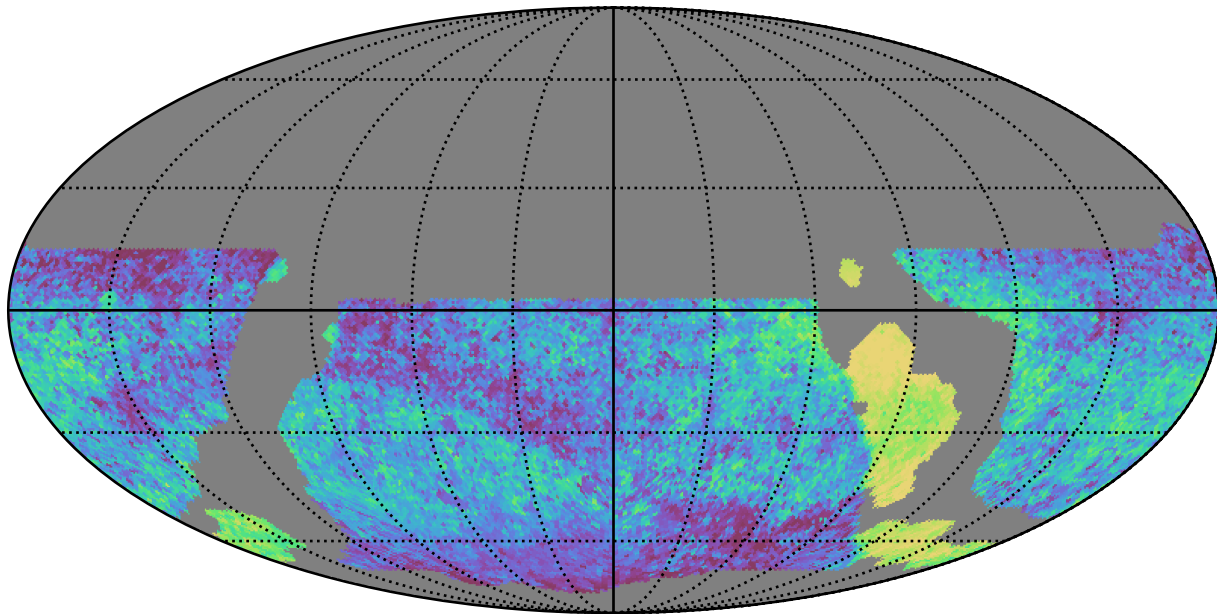
weather_cloudso12v3.4_10yrs WFD all bands: Median skyBrightness
