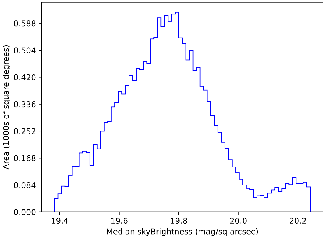
weather_cloudso12v3.4_10yrs WFD all bands: Median skyBrightness
