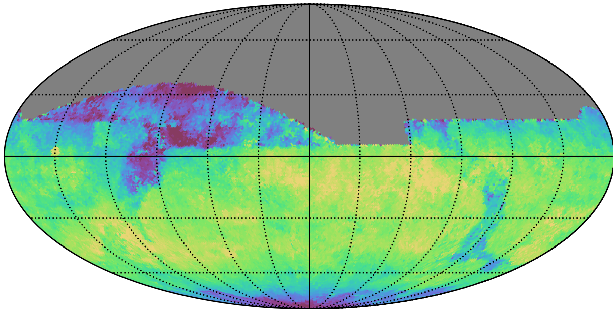
weather_cloudso12v3.4_10yrs All sky z band: Median skyBrightness
