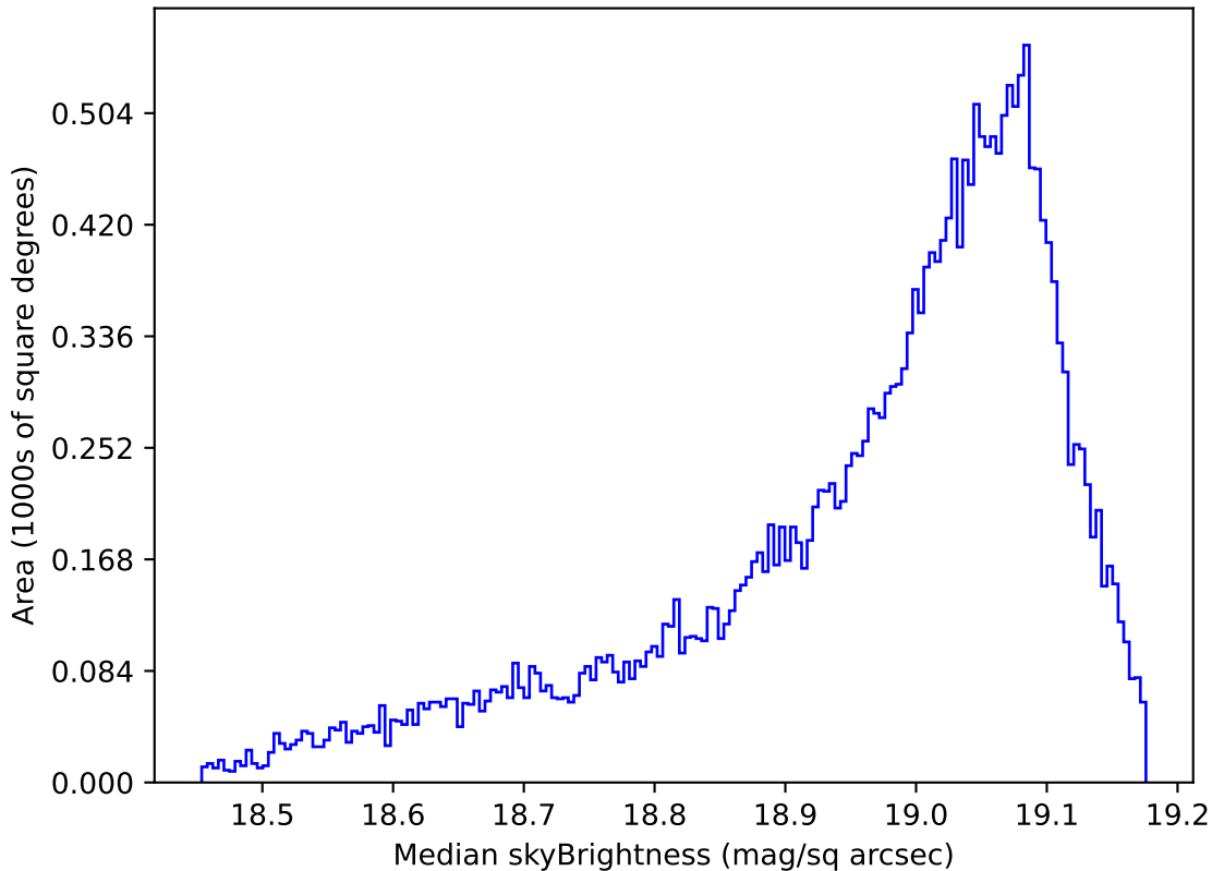
weather_cloudso12v3.4_10yrs All sky z band: Median skyBrightness
