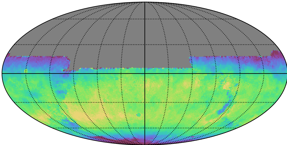
weather_cloudso12v3.4_10yrs All sky y band: Median skyBrightness
