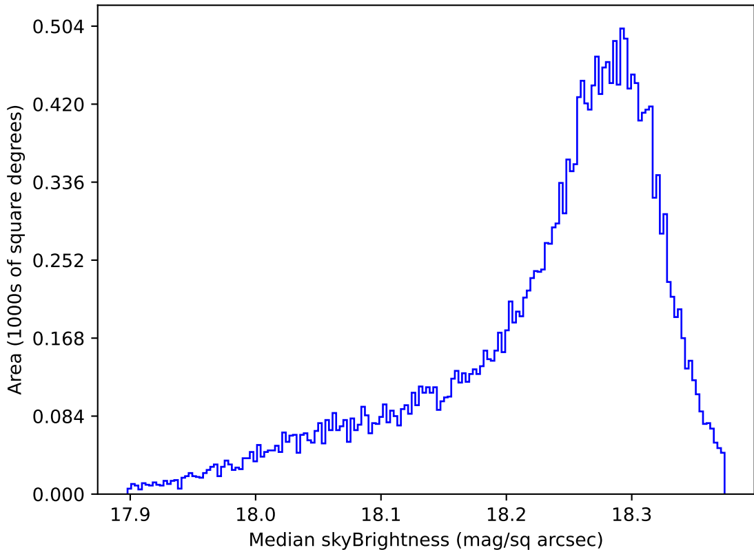
weather_cloudso12v3.4_10yrs All sky y band: Median skyBrightness
