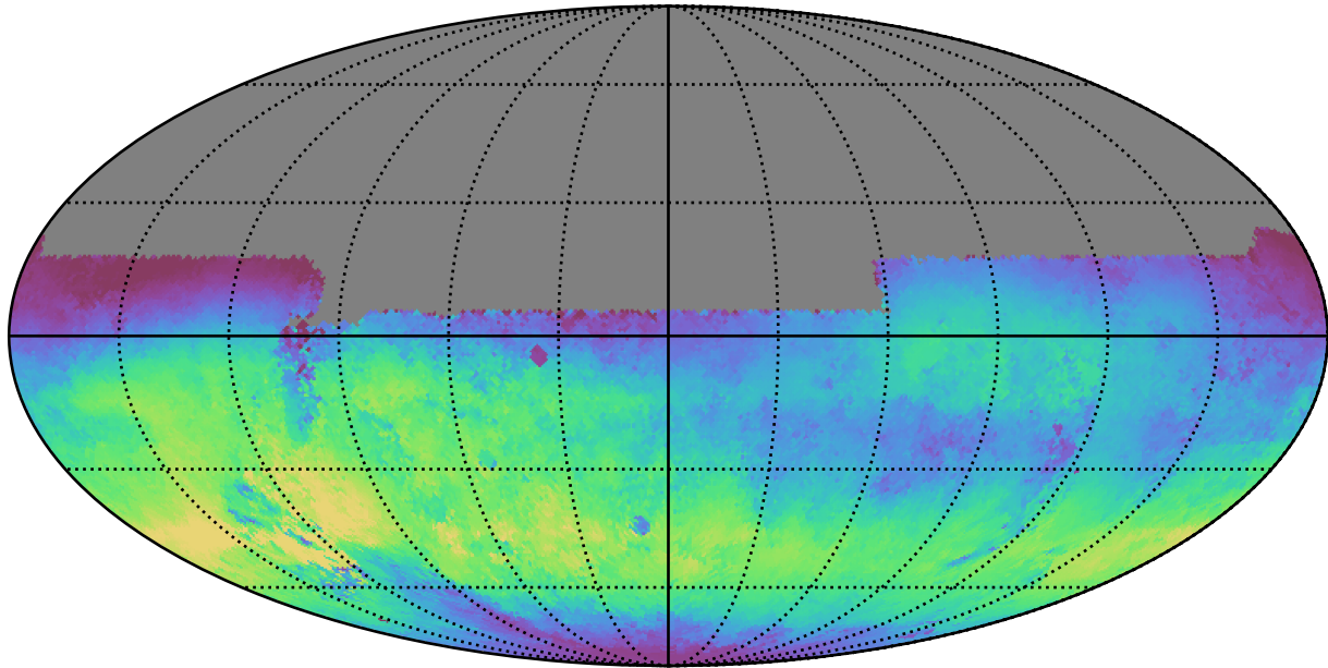
weather_cloudso12v3.4_10yrs All sky u band: Median skyBrightness
