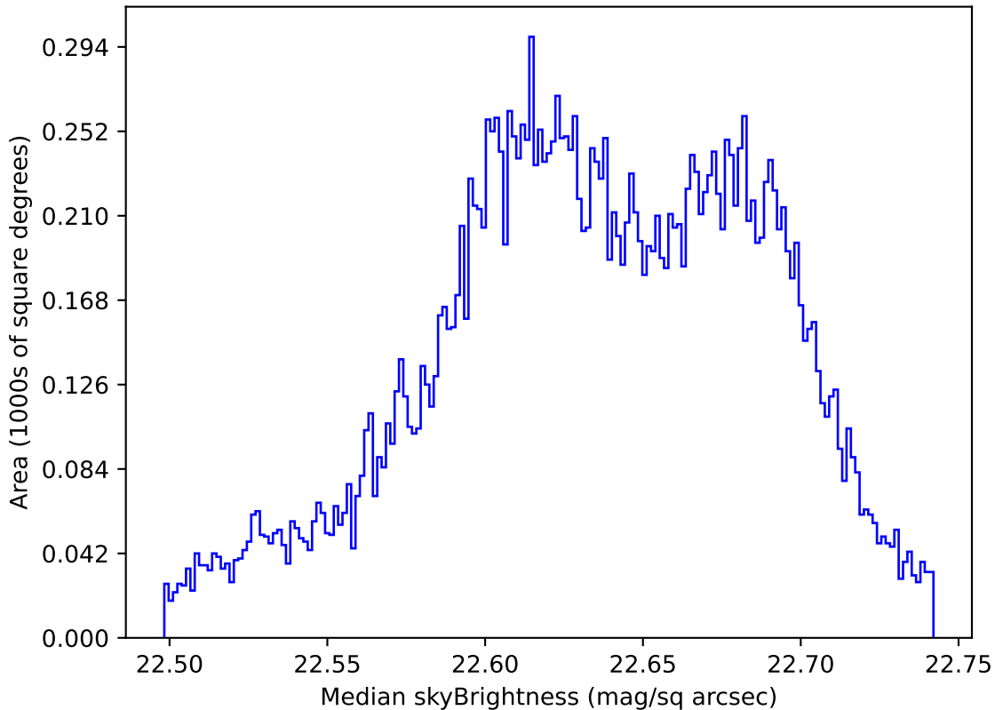
weather_cloudso12v3.4_10yrs All sky u band: Median skyBrightness
