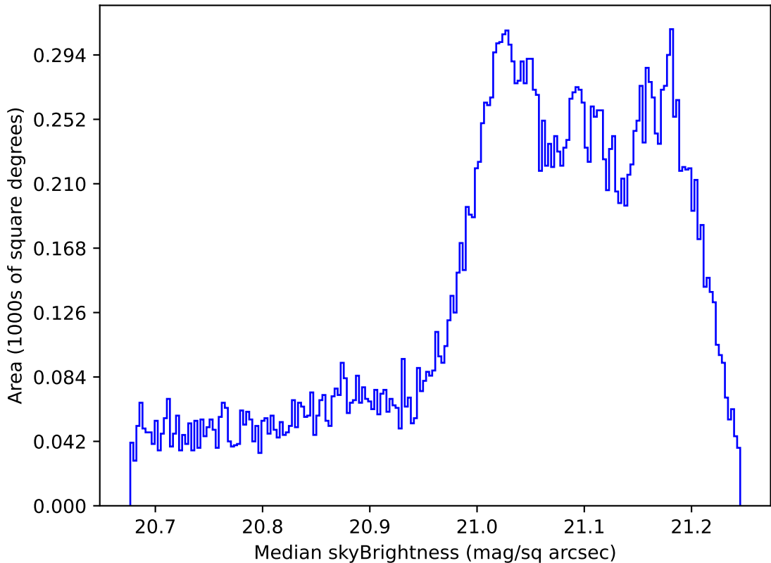
weather_cloudso12v3.4_10yrs All sky r band: Median skyBrightness
