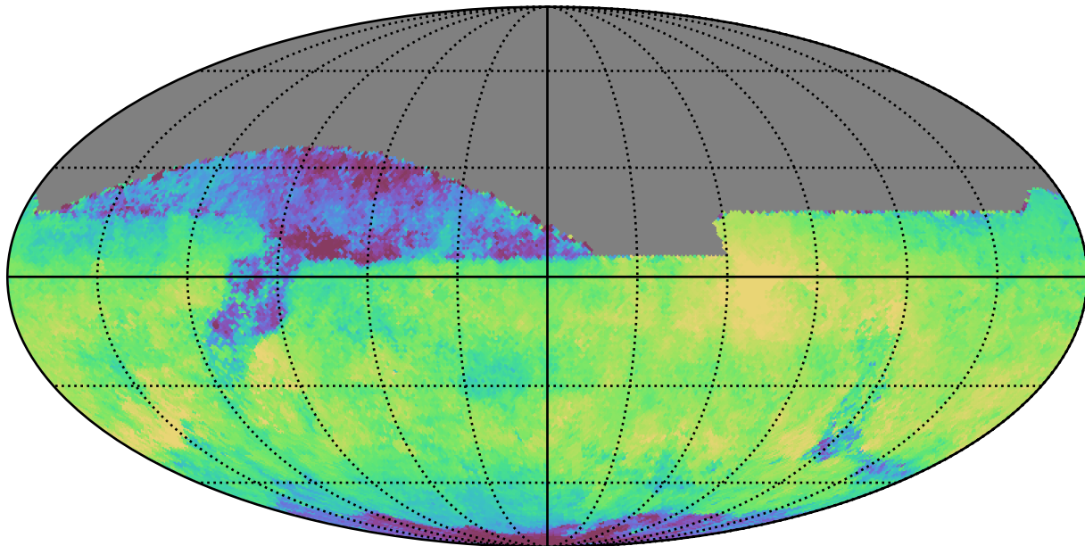
weather_cloudso12v3.4_10yrs All sky i band: Median skyBrightness
