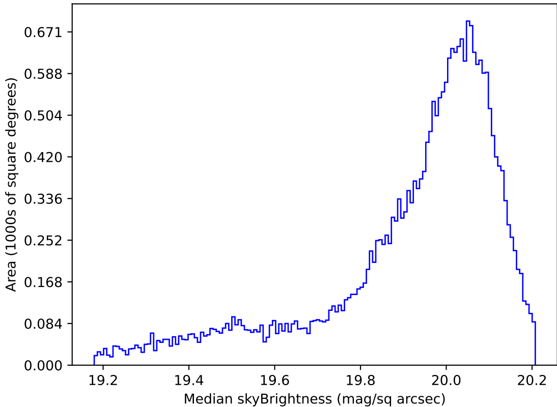
weather_cloudso12v3.4_10yrs All sky i band: Median skyBrightness
