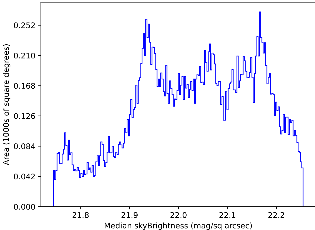
weather_cloudso12v3.4_10yrs All sky g band: Median skyBrightness
