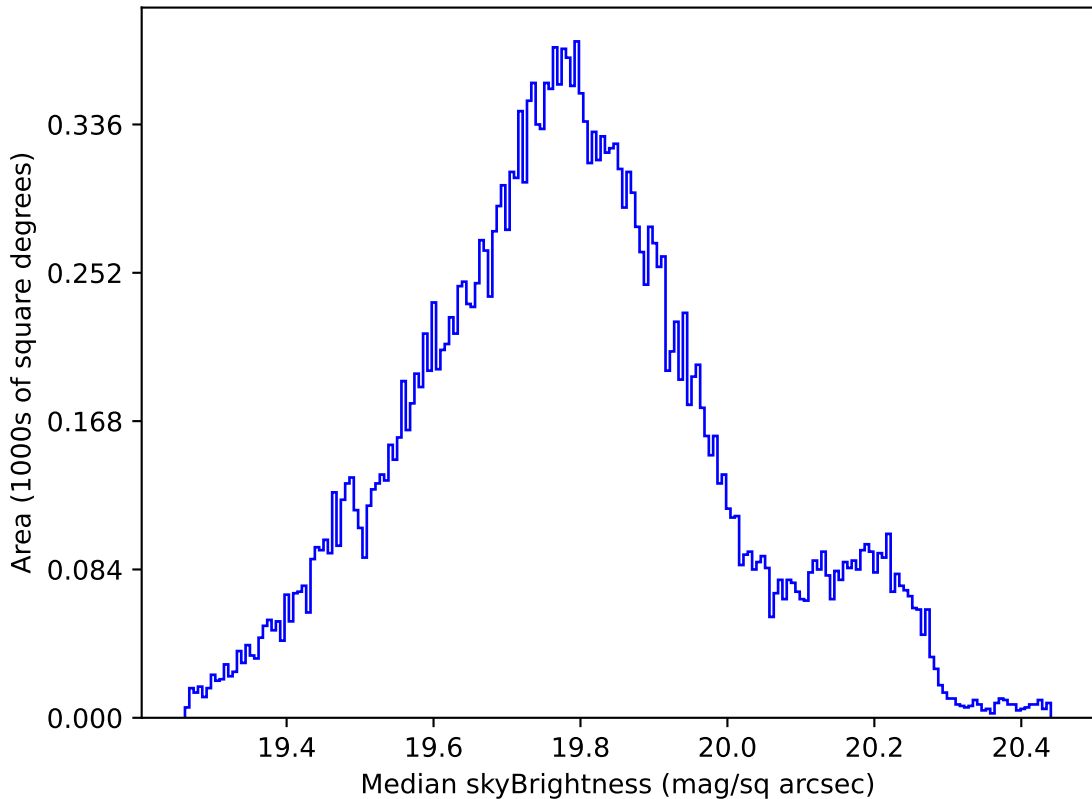
weather_cloudso12v3.4_10yrs All sky all bands: Median skyBrightness
