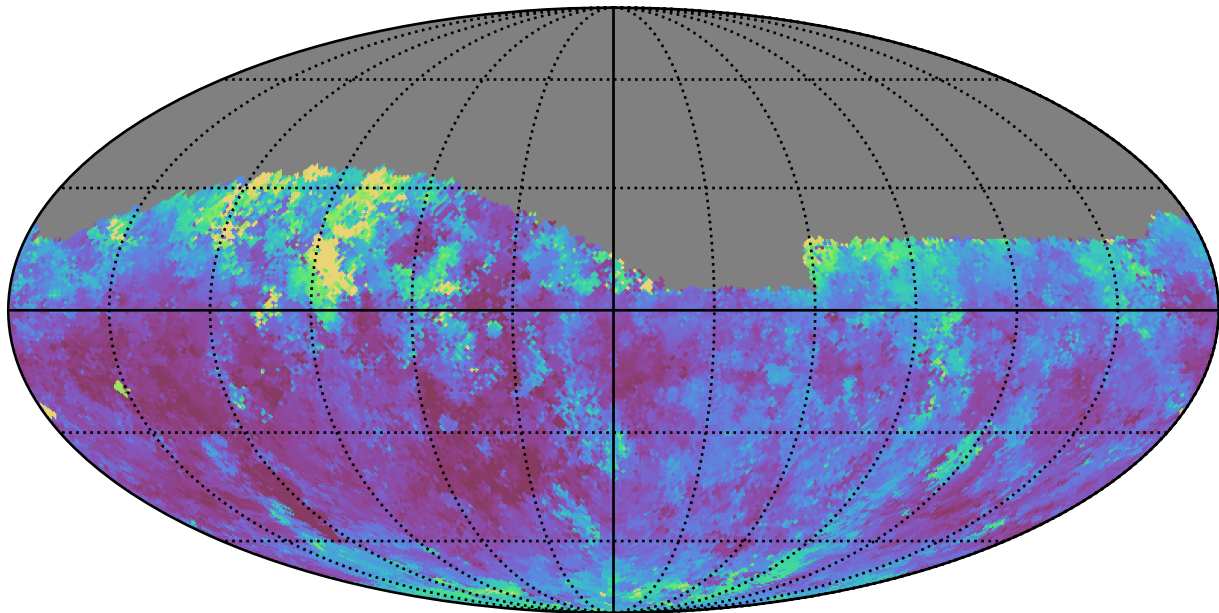
weather_cloudso12v3.4_10yrs Yr 1 z band: Median seeingGeom
