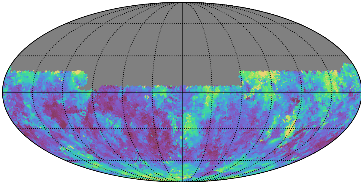
weather_cloudso12v3.4_10yrs Yr 1 y band: Median seeingGeom
