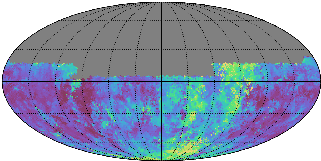
weather_cloudso12v3.4_10yrs Yr 1 u band: Median seeingGeom
