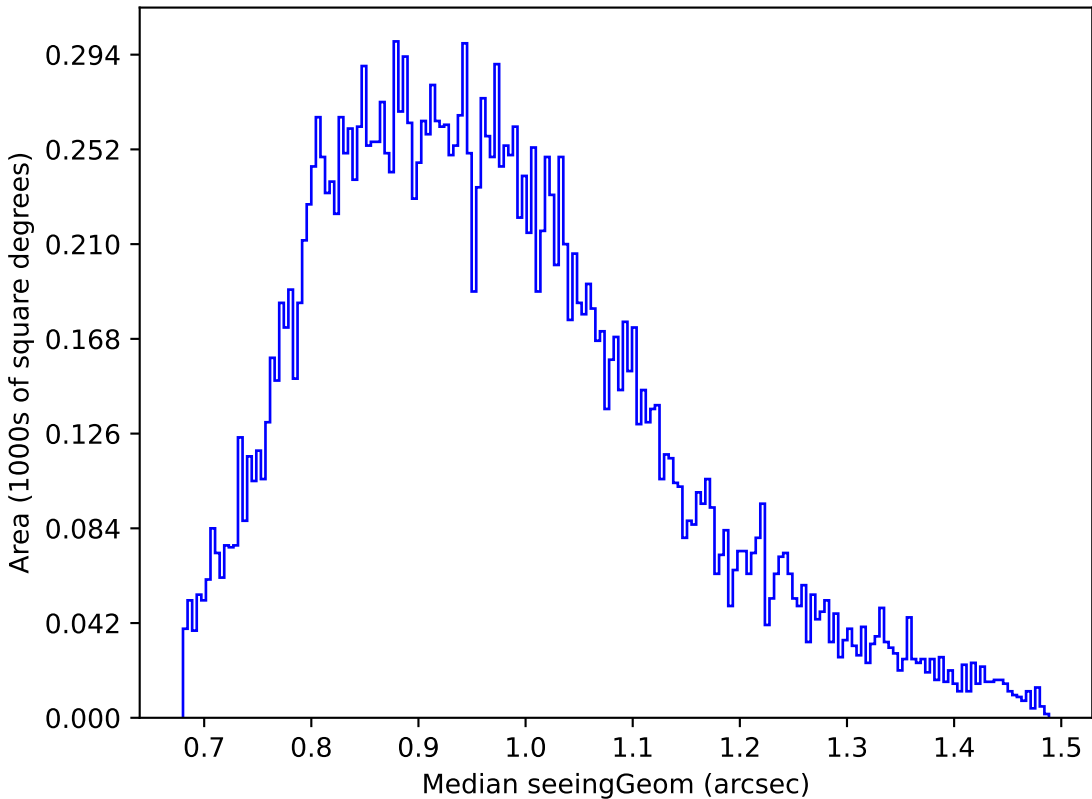
weather_cloudso12v3.4_10yrs Yr 1 u band: Median seeingGeom
