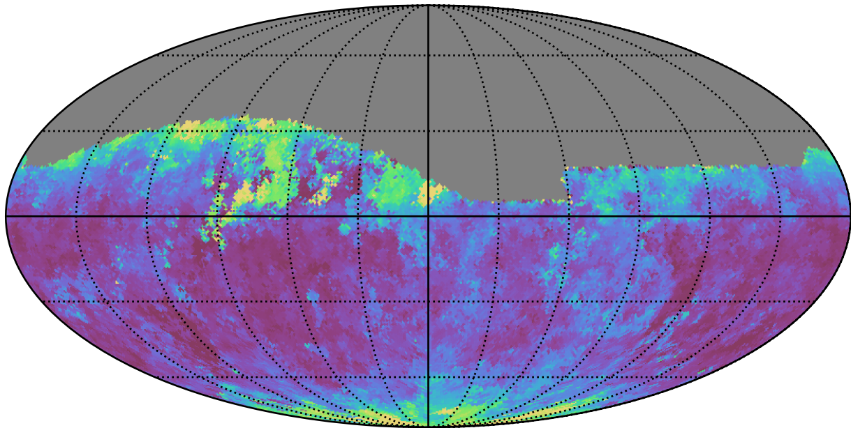
weather_cloudso12v3.4_10yrs Yr 1 r band: Median seeingGeom
