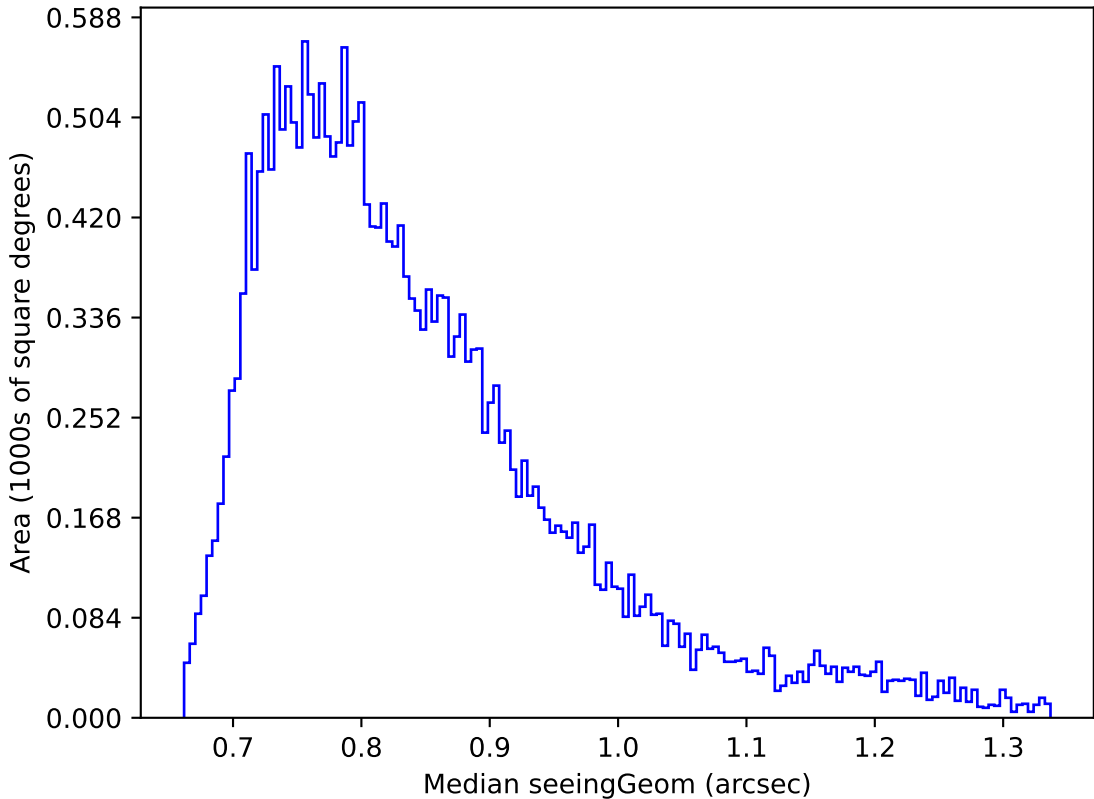
weather_cloudso12v3.4_10yrs Yr 1 r band: Median seeingGeom
