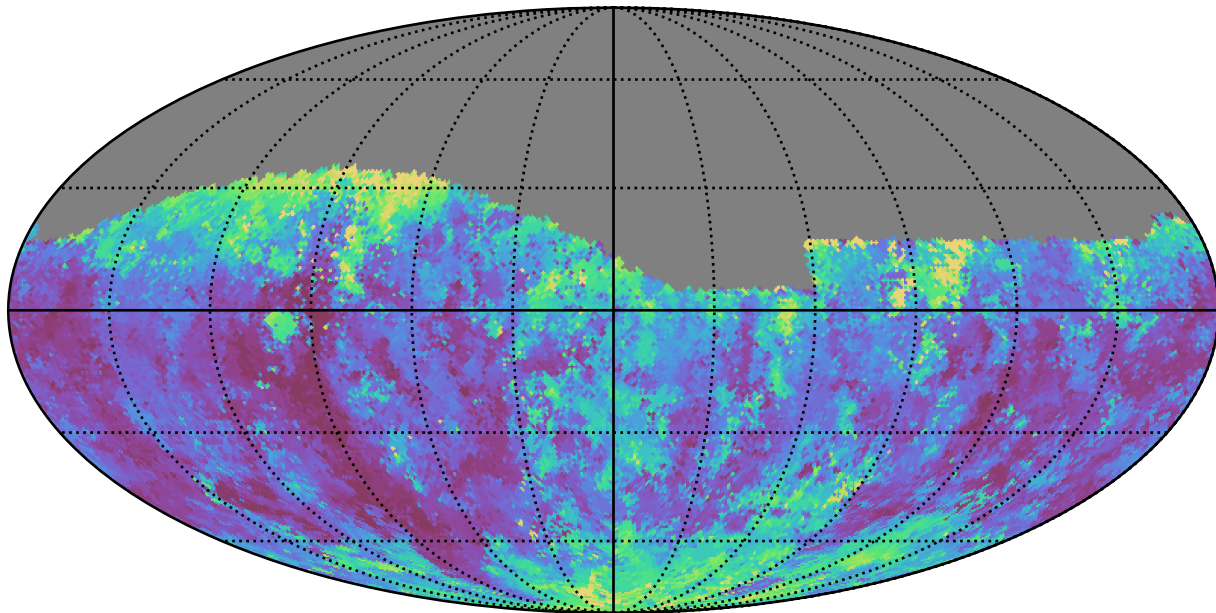
weather_cloudso12v3.4_10yrs Yr 1 g band: Median seeingGeom
