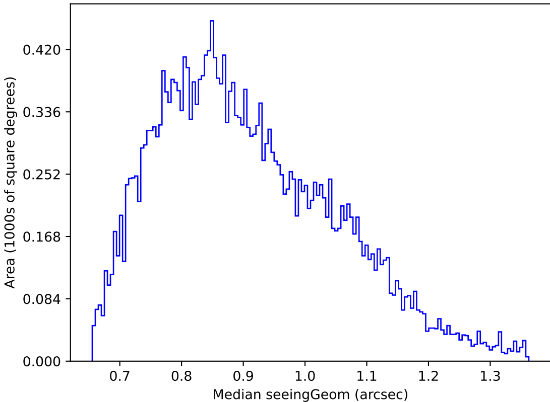
weather_cloudso12v3.4_10yrs Yr 1 g band: Median seeingGeom
