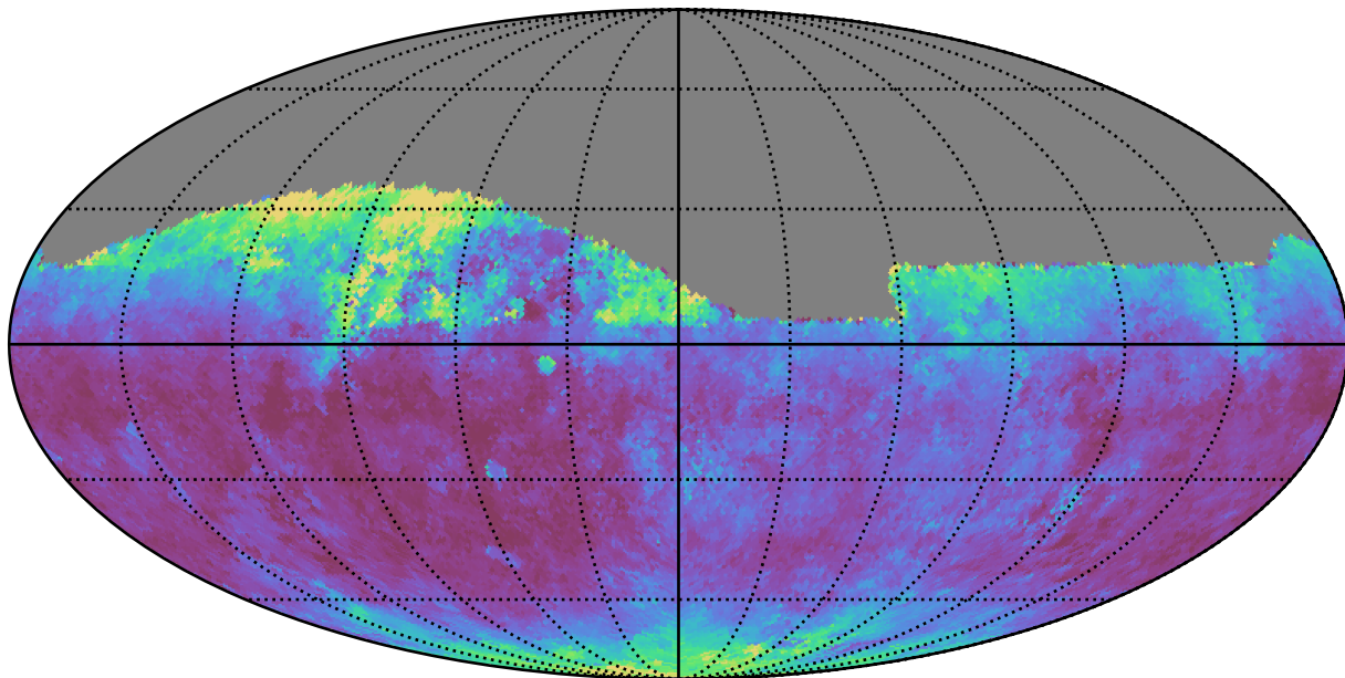
weather_cloudso12v3.4_10yrs Yr 1 all bands: Median seeingGeom
