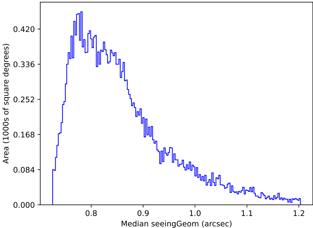
weather_cloudso12v3.4_10yrs Yr 1 all bands: Median seeingGeom
