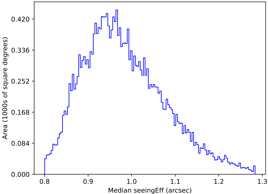
weather_cloudso12v3.4_10yrs Yr 1 y band: Median seeingEff
