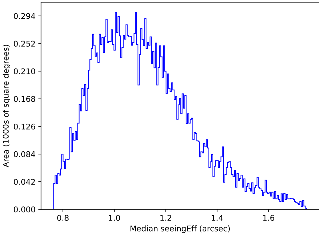
weather_cloudso12v3.4_10yrs Yr 1 u band: Median seeingEff
