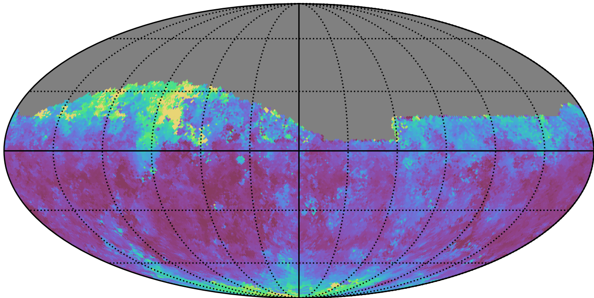
weather_cloudso12v3.4_10yrs Yr 1 i band: Median seeingEff
