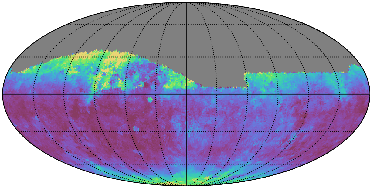
weather_cloudso12v3.4_10yrs Yr 1 all bands: Median seeingEff
