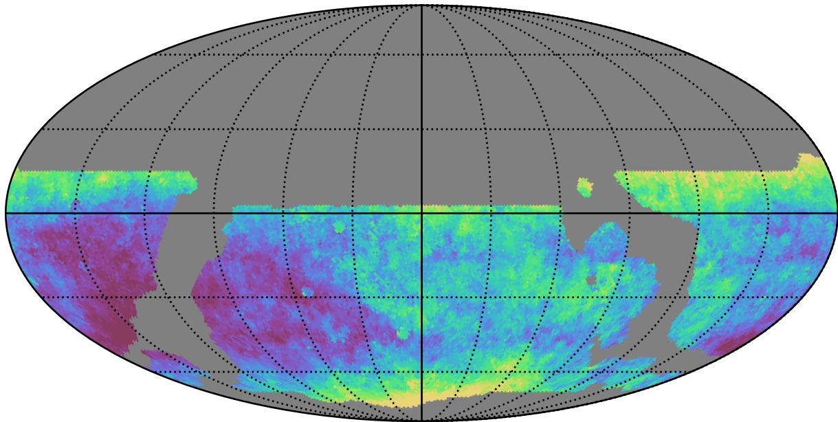
weather_cloudso12v3.4_10yrs WFD z band: Median seeingEff
