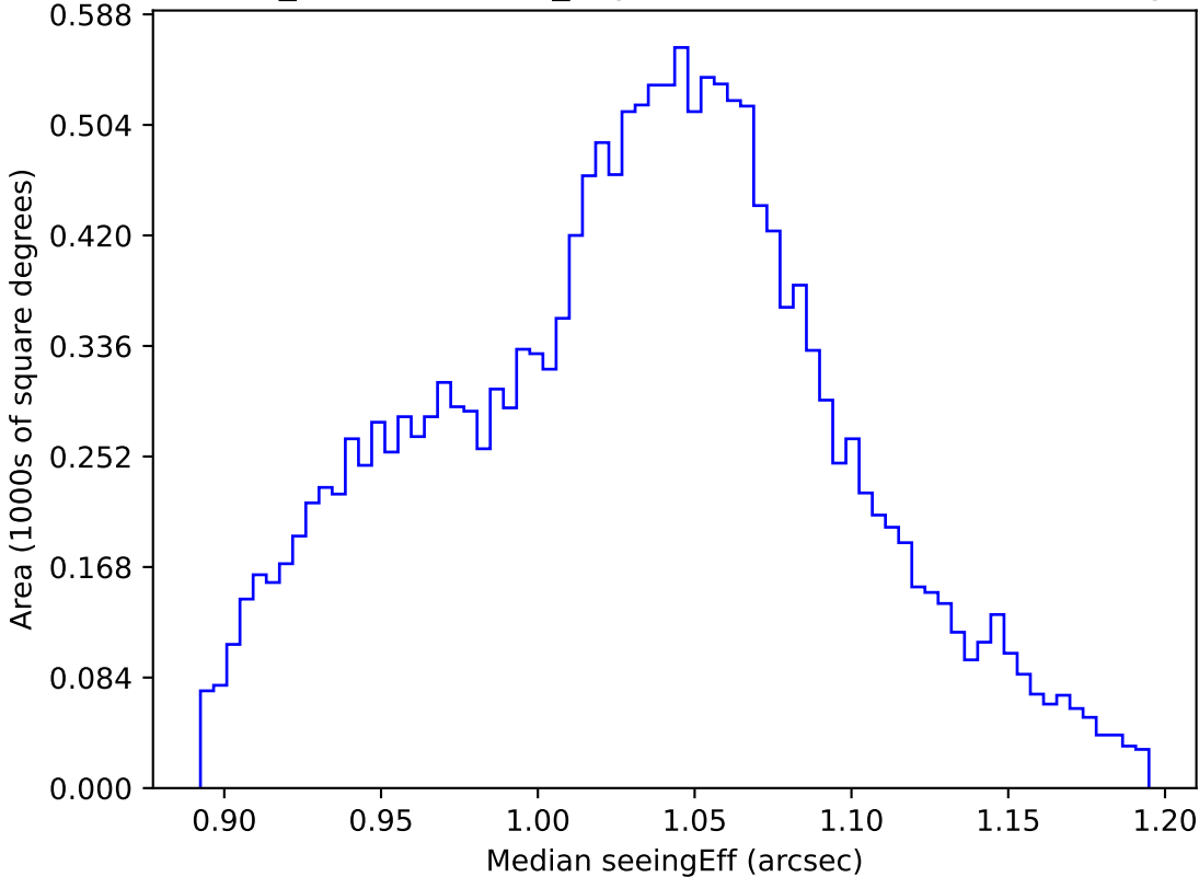
weather_cloudso12v3.4_10yrs WFD z band: Median seeingEff
