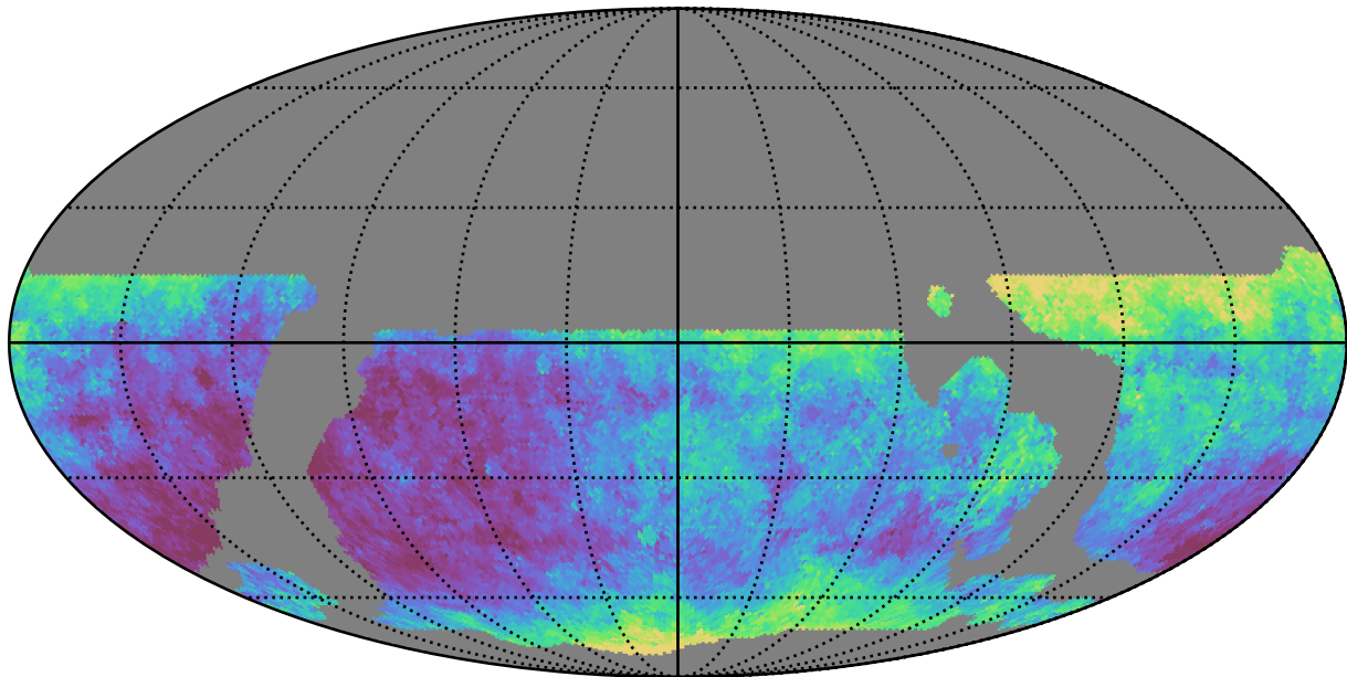
weather_cloudso12v3.4_10yrs WFD y band: Median seeingEff
