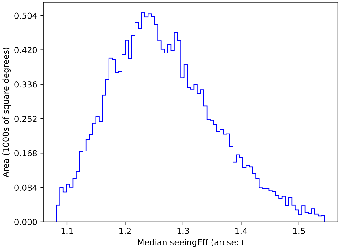
weather_cloudso12v3.4_10yrs WFD u band: Median seeingEff
