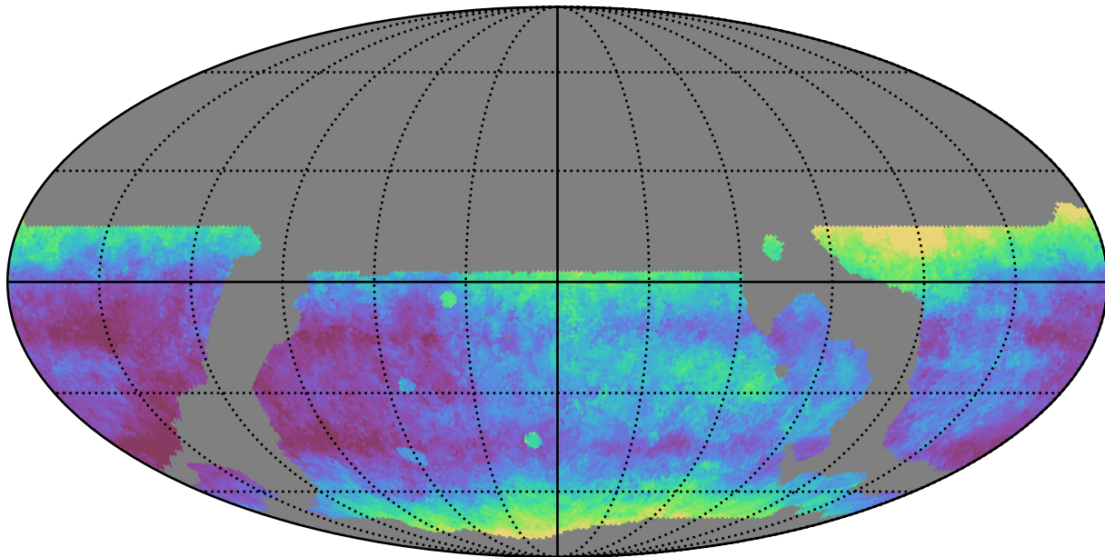
weather_cloudso12v3.4_10yrs WFD r band: Median seeingEff
