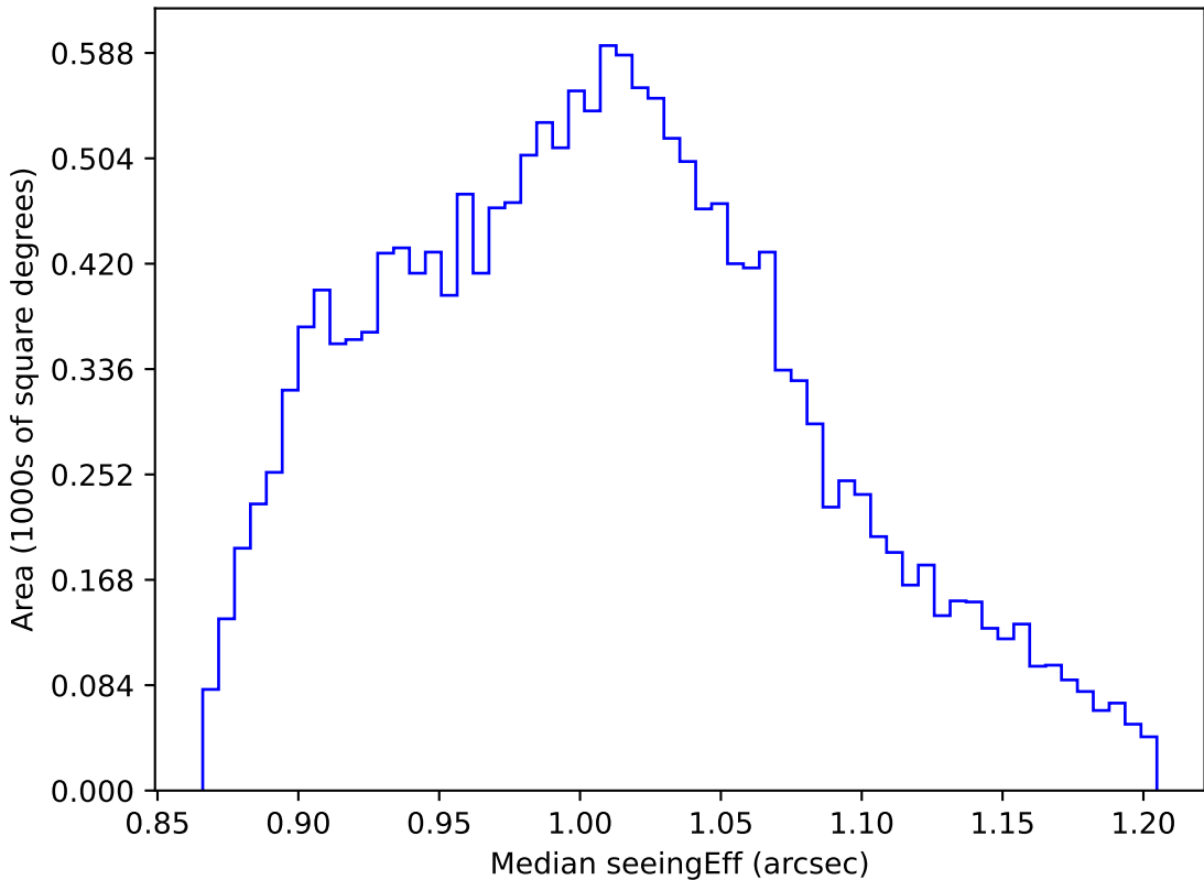
weather_cloudso12v3.4_10yrs WFD i band: Median seeingEff
