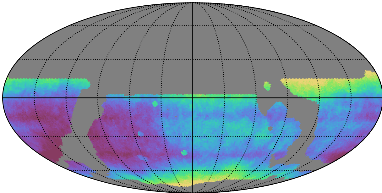
weather_cloudso12v3.4_10yrs WFD all bands: Median seeingEff
