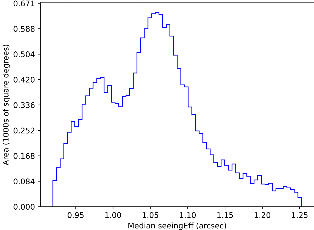
weather_cloudso12v3.4_10yrs WFD all bands: Median seeingEff
