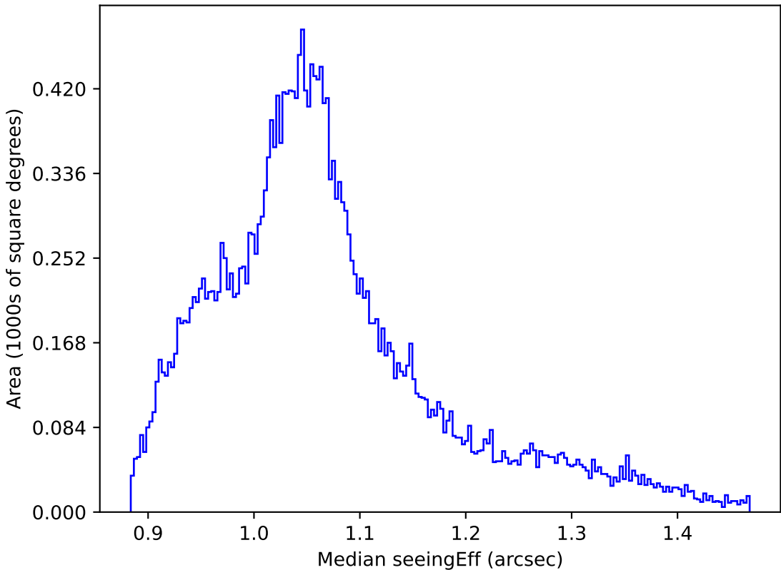
weather_cloudso12v3.4_10yrs All sky z band: Median seeingEff
