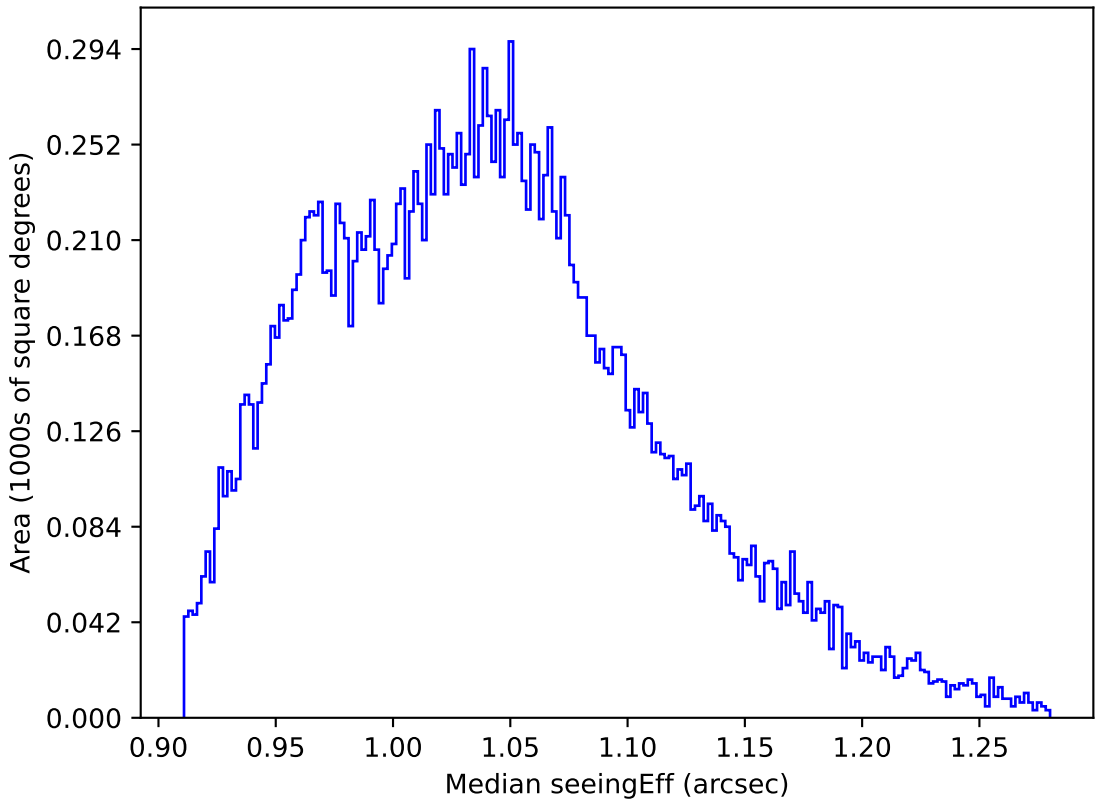
weather_cloudso12v3.4_10yrs All sky y band: Median seeingEff
