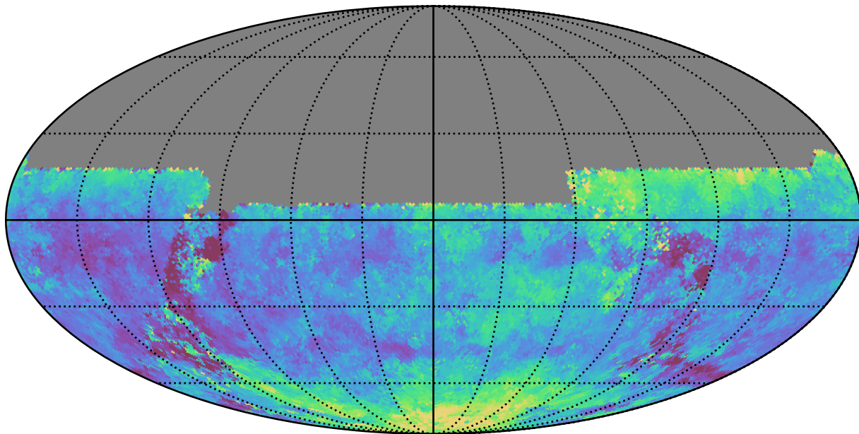
weather_cloudso12v3.4_10yrs All sky u band: Median seeingEff
