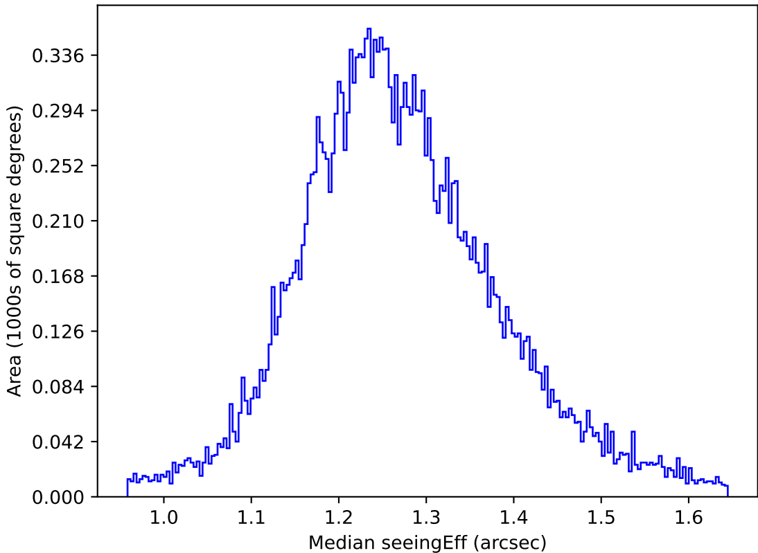
weather_cloudso12v3.4_10yrs All sky u band: Median seeingEff
