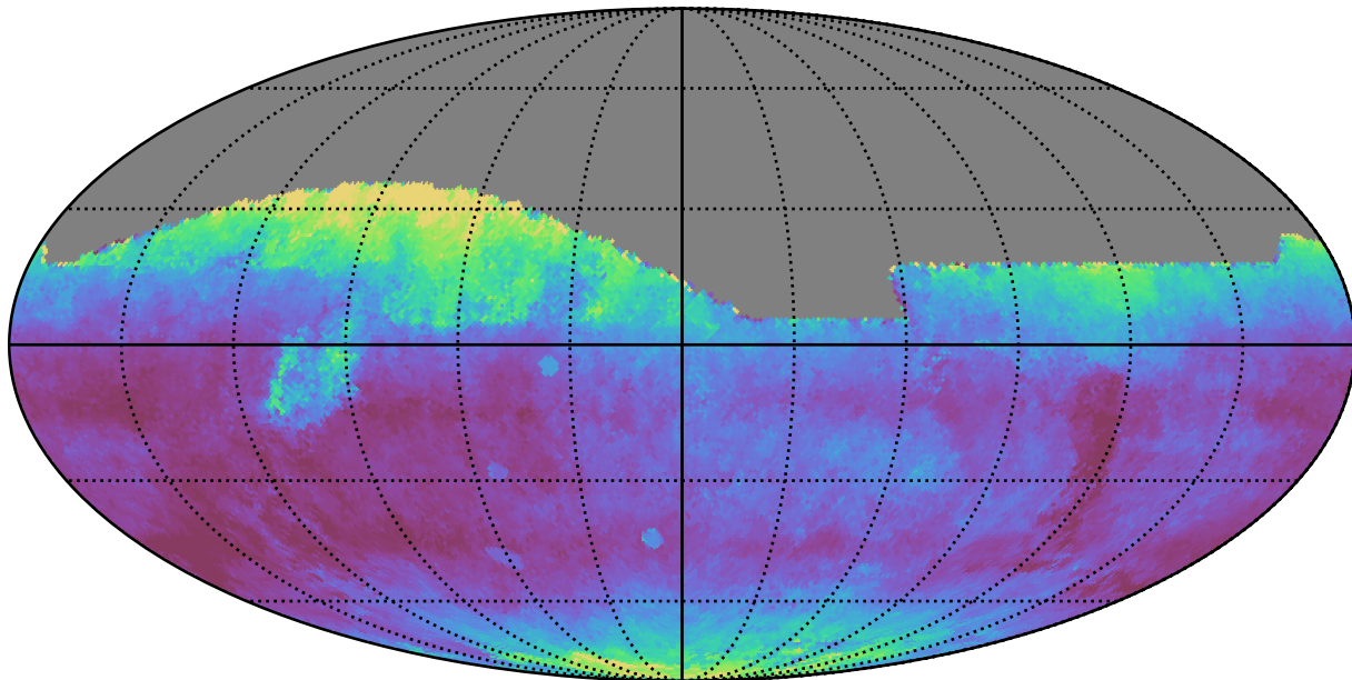
weather_cloudso12v3.4_10yrs All sky r band: Median seeingEff
