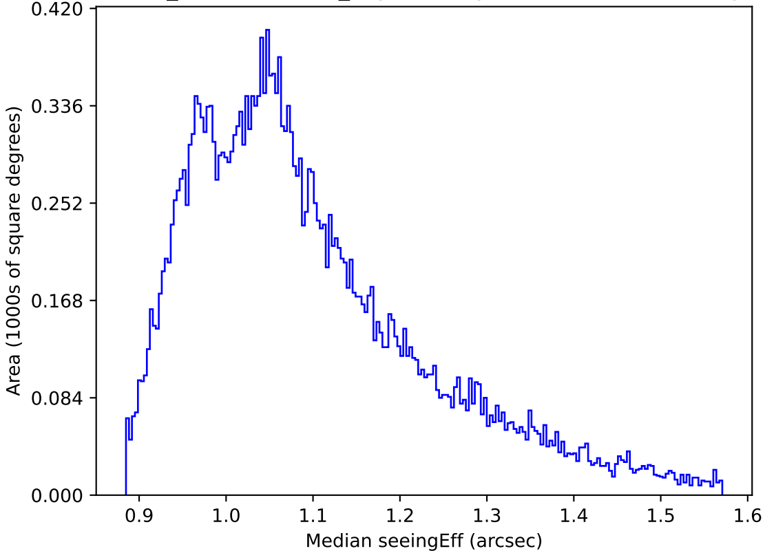
weather_cloudso12v3.4_10yrs All sky r band: Median seeingEff
