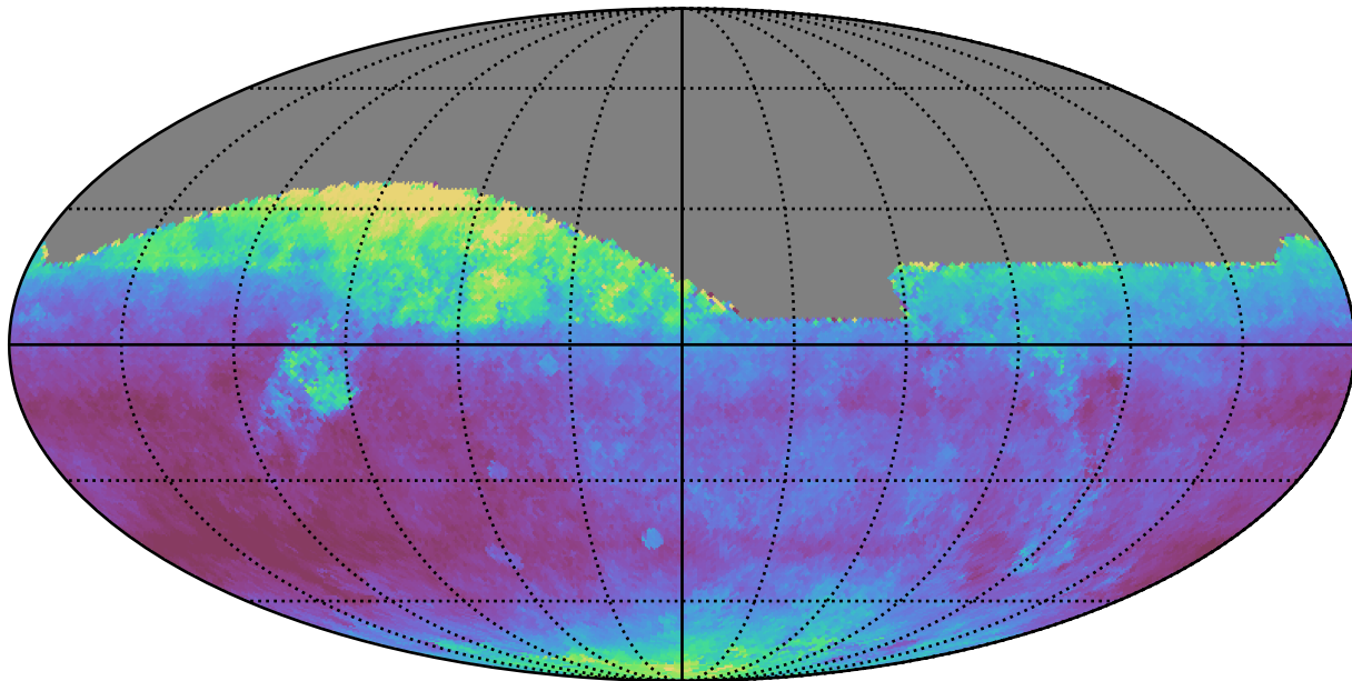
weather_cloudso12v3.4_10yrs All sky i band: Median seeingEff
