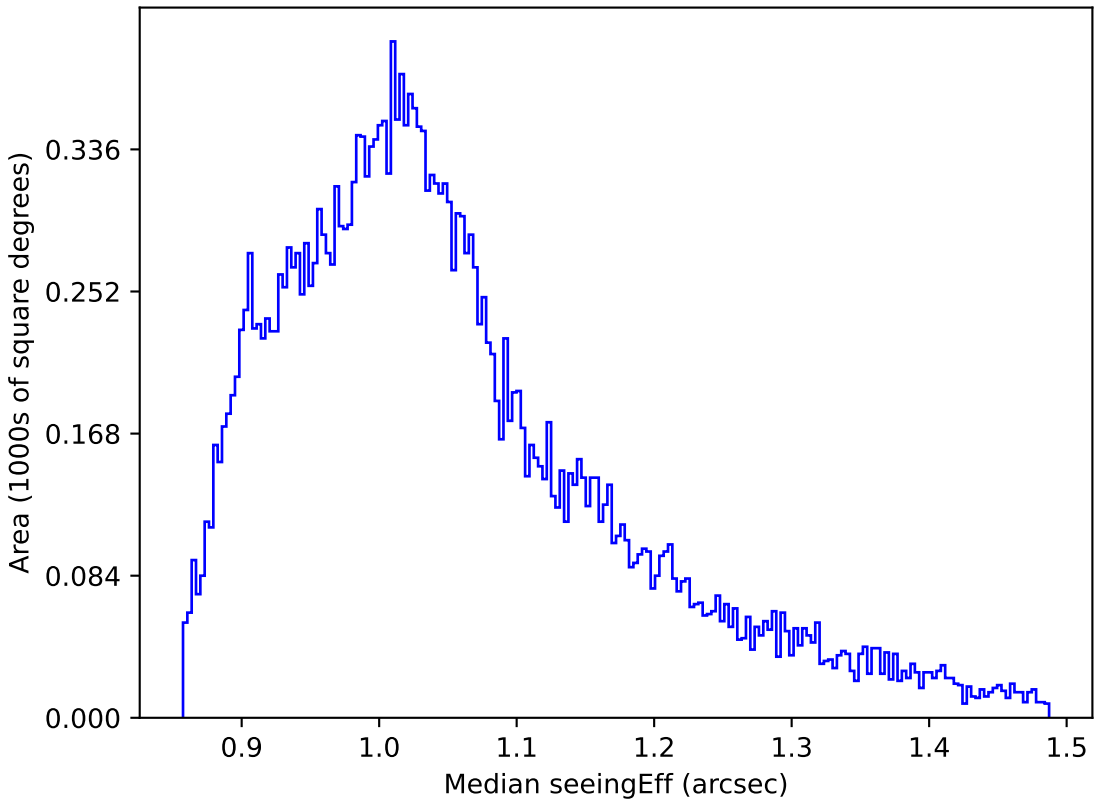
weather_cloudso12v3.4_10yrs All sky i band: Median seeingEff
