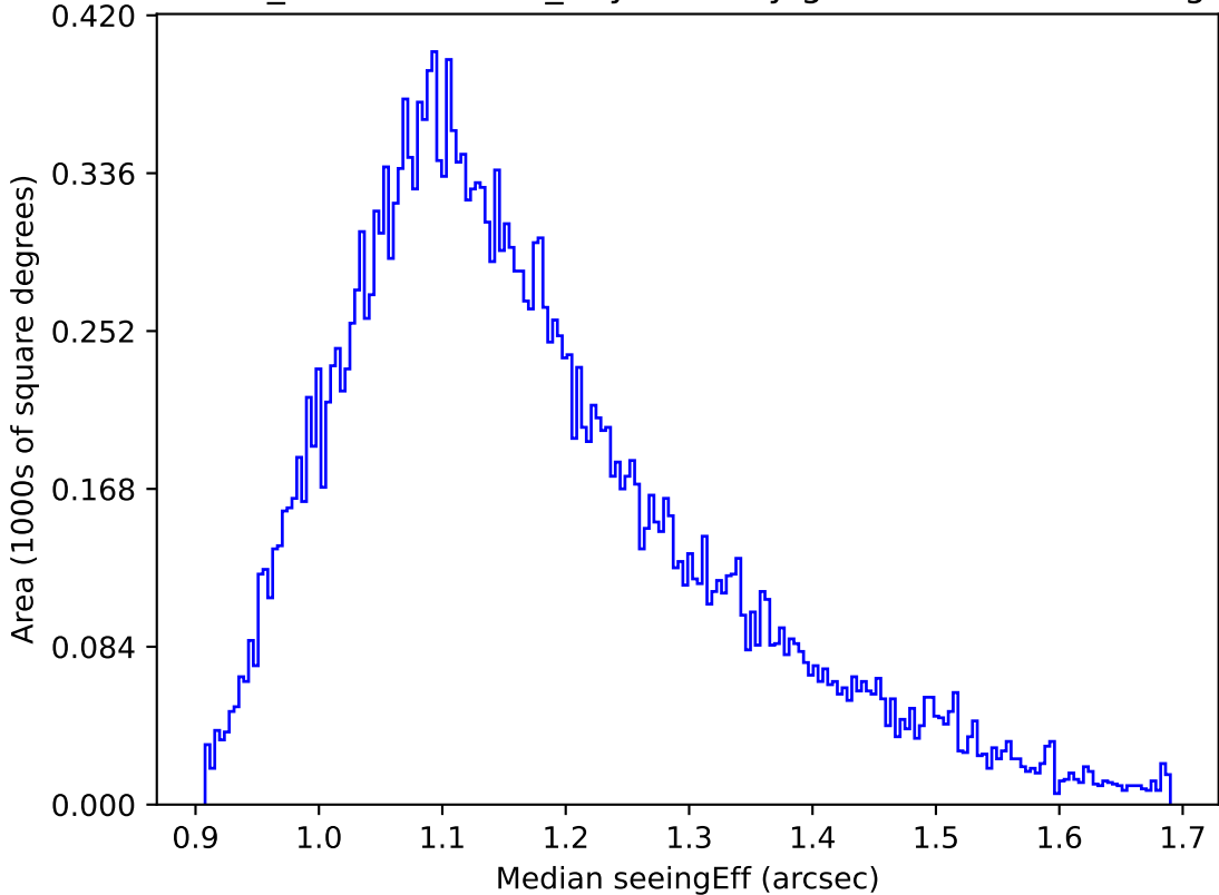
weather_cloudso12v3.4_10yrs All sky g band: Median seeingEff
