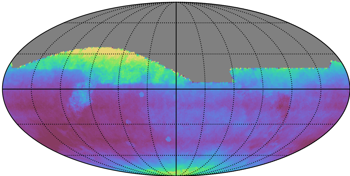
weather_cloudso12v3.4_10yrs All sky all bands: Median seeingEff
