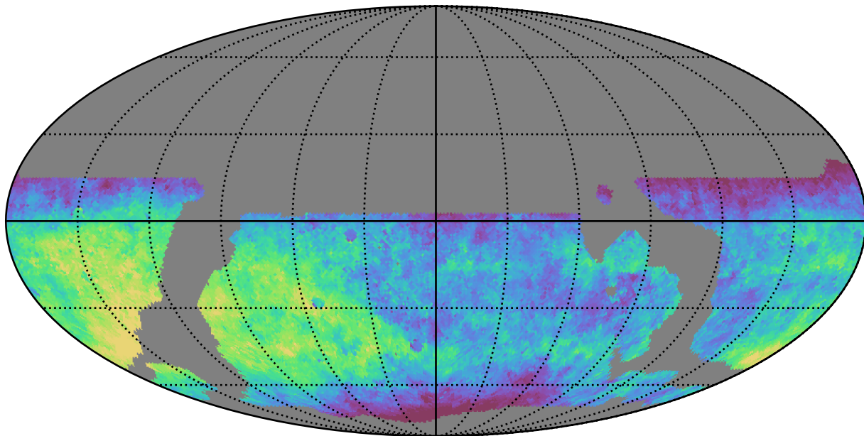
weather_cloudso12v3.4_10yrs WFD z band: Median saturation_mag
