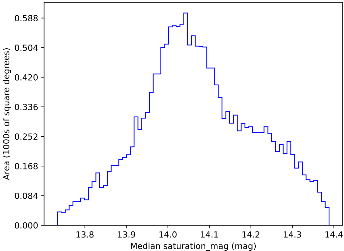
weather_cloudso12v3.4_10yrs WFD z band: Median saturation_mag
